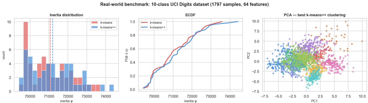
Figure 10: Real-world benchmark: UCI Digits. Left: inertia histogram. Middle: ECDF. Right: PCA projection of the best k -means ++ clustering.
